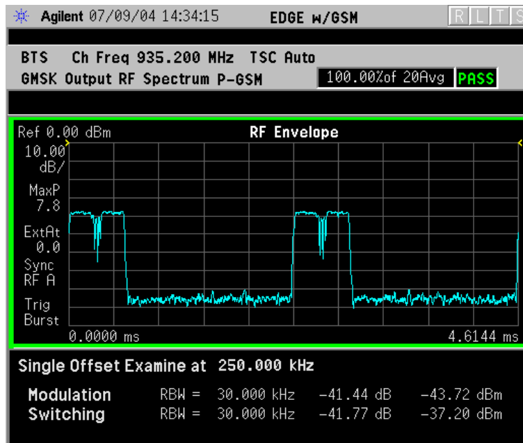
Figure 2-28 GSMK ORFS Result - Switching Single Offset (Examine) View
